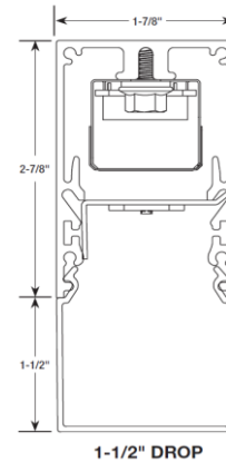
Luminaire Cross Section
